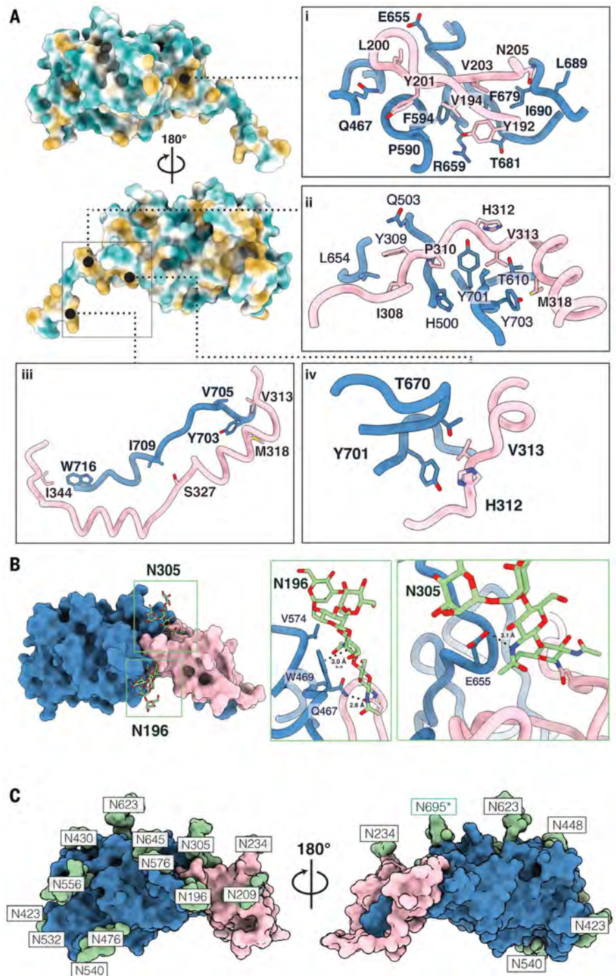
Fig. 3. The E1E2 interface and glycan shield. (A) The newly characterized E1E2 interface is stabilized by hydrophobic interactions. E2 is colored by hydrophobicity, with green representing hydrophilic regions and yellow signifying hydrophobic patches. The first panel (i) showcases a deep hydrophobic cavity in the base of E2 against which E1 packs. The following panels (ii to iv) highlight additional hydrophobic interactions that we assert further stabilize the E1E2 interface. (B) Glycans buttress the E1E2 interface. Key interactions between glycans N196 and N305 are showcased. Glycan N196 is involved in hydrophobic interactions, including a \pi - \pi stacking interaction with W469, as well as a salt bridge with Q467. N305 forms a stabilizing salt bridge with E655. (C) Surface representation of the E1 and E2 model showing the glycan sites in green with their respective asparagine residues. The predominant glycoform identified by LC-MS at each PNGS was modeled using Coot (59). An asterisk indicates that the glycan at position N695 uses a noncanonical N-glycosylation motif, NXV. Single-letter abbreviations for the amino acid residues are as follows: A, Ala; C, Cys; D, Asp; E, Glu; F, Phe; G, Gly; H, His; I, Ile; K, Lys; L, Leu; M, Met; N, Asn; P, Pro; Q, Gln; R, Arg; S, Ser; T, Thr; V, Val; W, Trp; and Y, Tyr.
