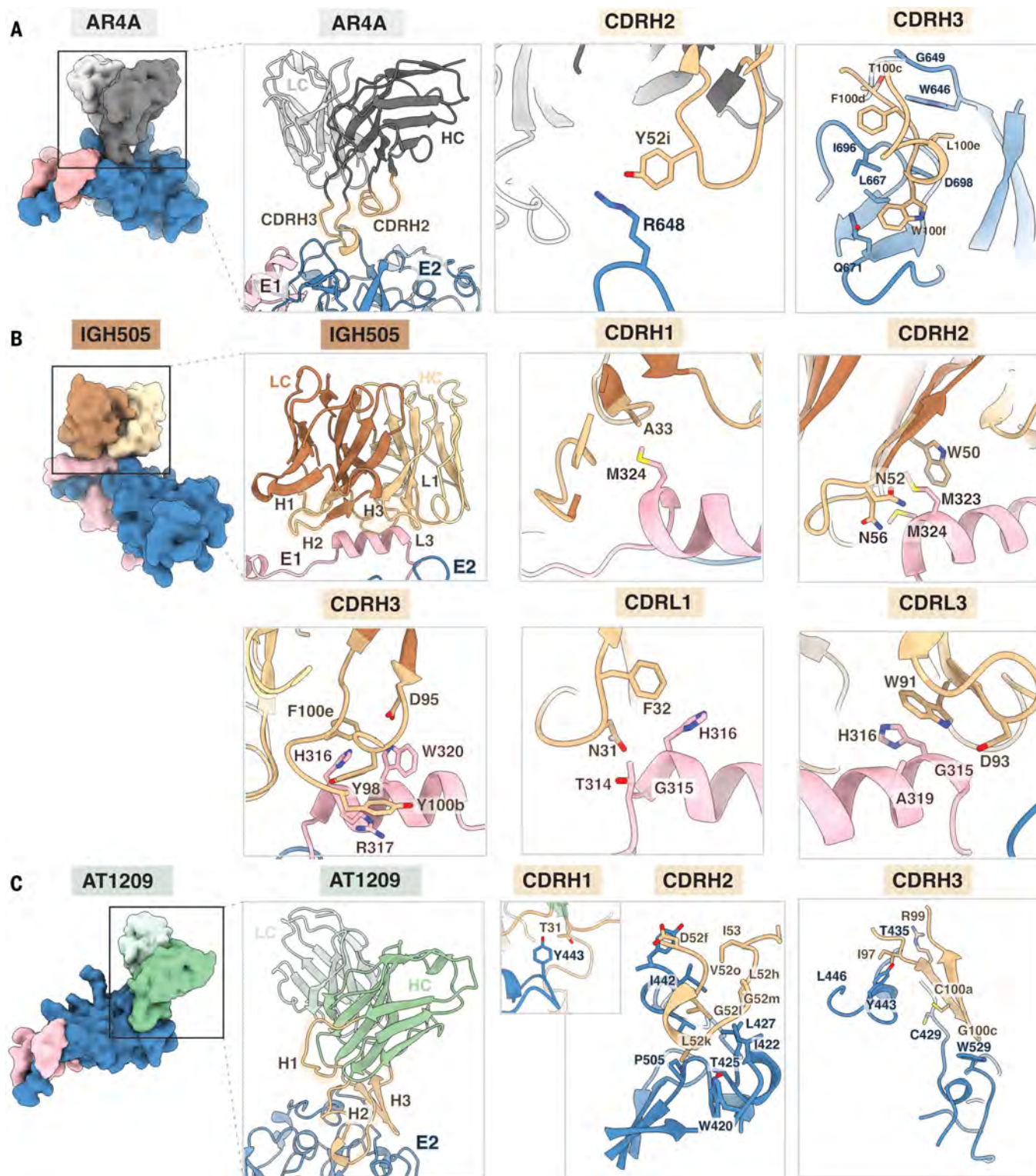
Fig. 4. Structural definition of the AR4A, IGH505, and AT1209 epitopes. (A) The AR4A Fab recognizes protein elements in E2 (blue) near the interface with the E1 subunit (pink). Heavy and light chains are shown in dark and light gray, respectively, and CDRH2 and CDRH3 are highlighted in tan. Whereas the CDRH2 only interacts with the stem region of E2, the CDRH3 loop targets both the back layer and stem of E2. (B) The IGH505 Fab interacts with the surface-exposed \alpha helix in E1 (pink). Heavy and light chains are shown in brown and yellow, respectively, and CDRH1 to CDRH3 and CDRL1 and CDRL3 are
